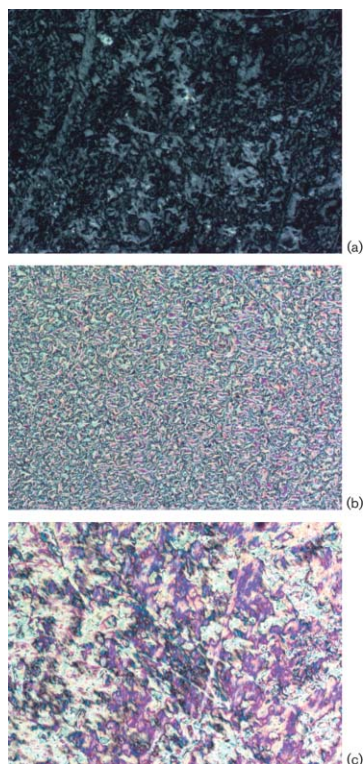
Fig. 3 Photomicrographs, taken over <0.5 °C, of the N-SmC transition of 6-16 : (a) nematic, (b) transition, (c) SmC phase.
